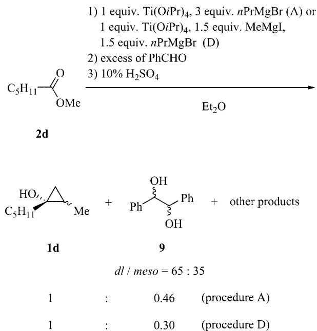
Scheme 11. Trapping of titanium(III) alkoxides with \text{PhCHO} .
