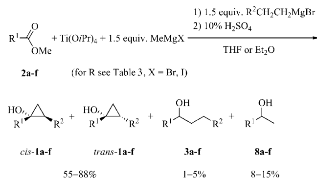
Scheme 9. Advanced procedure for the preparation of 1,2-disubstituted cyclopropanols.
