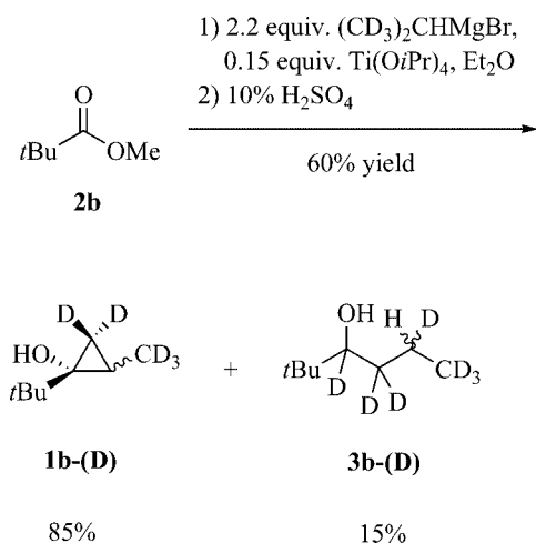
Scheme 4. Cyclopropanation of methyl pivalate ( 2b ) with (CD 3 ) 2 CHMgBr.
