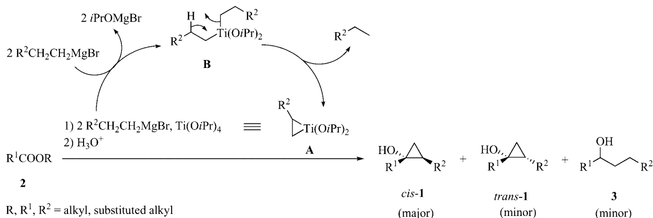
Scheme 1. Synthesis of 1,2-disubstituted cyclopropanols.
