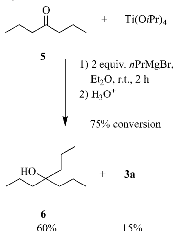
Scheme 3. Reaction between ketone 5 and 2 equiv. n PrMgBr and 1 equiv. Ti(O i Pr) 4 .
