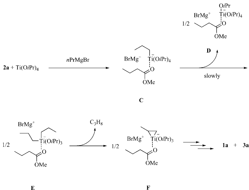
Scheme 5. Reaction between ester 2a and 1 equiv. of n PrMgBr and 1 equiv. of \text{Ti}(\text{OiPr})_4 .
