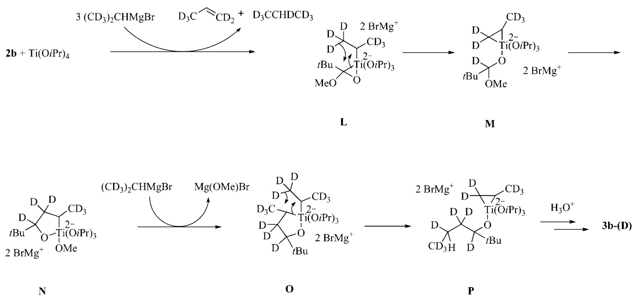
Scheme 8. Proposed mechanism for the formation of alcohol 3b-(D) .
