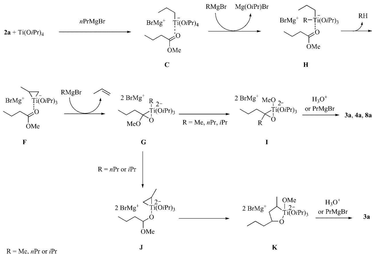
Scheme 7. Proposed mechanism for the formation of secondary alcohols 3a , 4a , and 8a .
