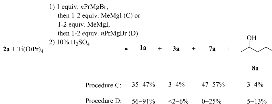
Scheme 6. Cyclopropanation of methyl butyrate ( 2a ) with n PrMgBr and MeMgI.
