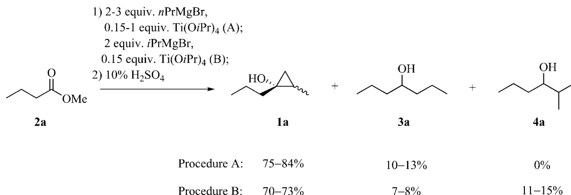
Scheme 2. Cyclopropanation of methyl butyrate ( 2a ).
